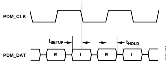
Figure 11. PDM Timing Diagram
